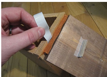
Figure 4 Slide the camera cable between the roof hinge and the back wall of the box
