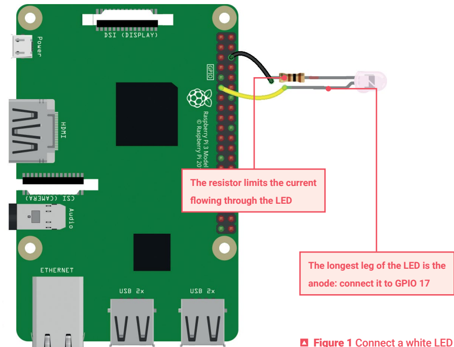
Figure 1 Connect a white LED
