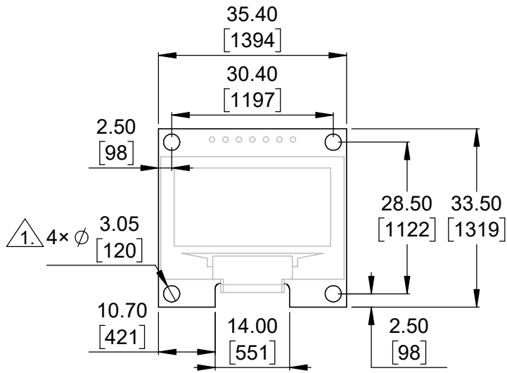
① Board dimensions (top view) Scale 1:1
