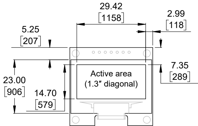
① Board dimensions (top view) Scale 1:1
