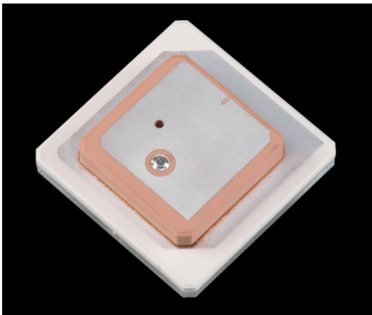
Figure 57: Ceramic Stack
