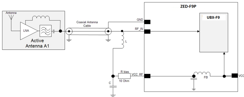
Figure 66: ZED-F9P VCC_RF antenna bias
