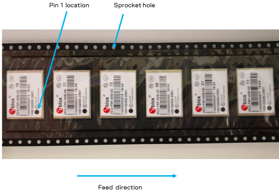
Figure 78: Orientation of ZED-F9P high precision receivers on the tape
