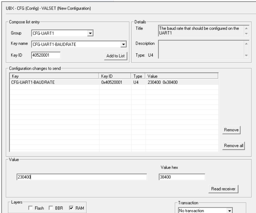
Figure 8: Base station: u-center UBX-CFG-VALSET message view for setting the CFG-UART1-BAUDRATE configuration item that controls the baudrate of UART1
