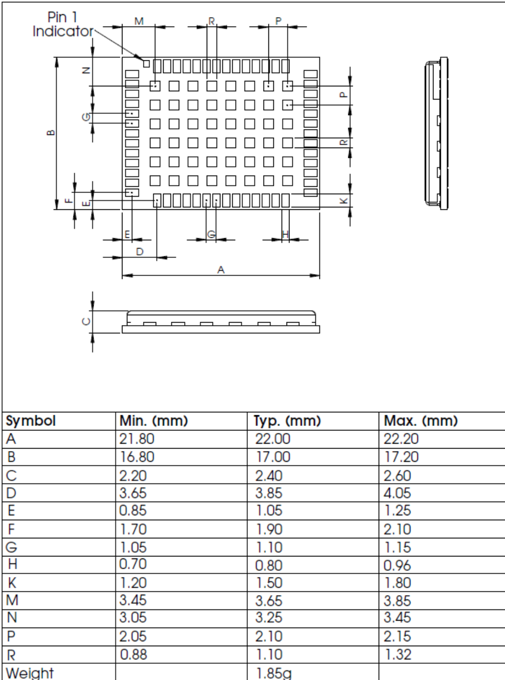
Figure 69: ZED-F9P LGA mechanical dimensions
