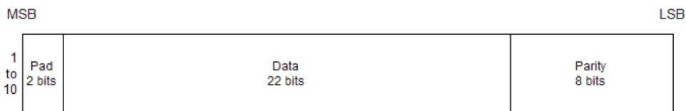
Figure 30: BeiDou subframe word
