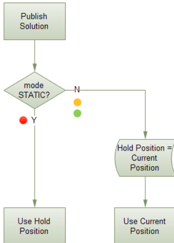
Figure 33: Position publication in static hold mode
