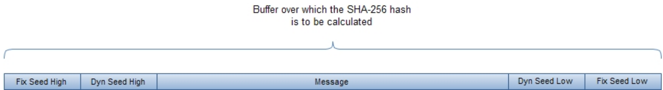
Figure 41: SHA256 hash
