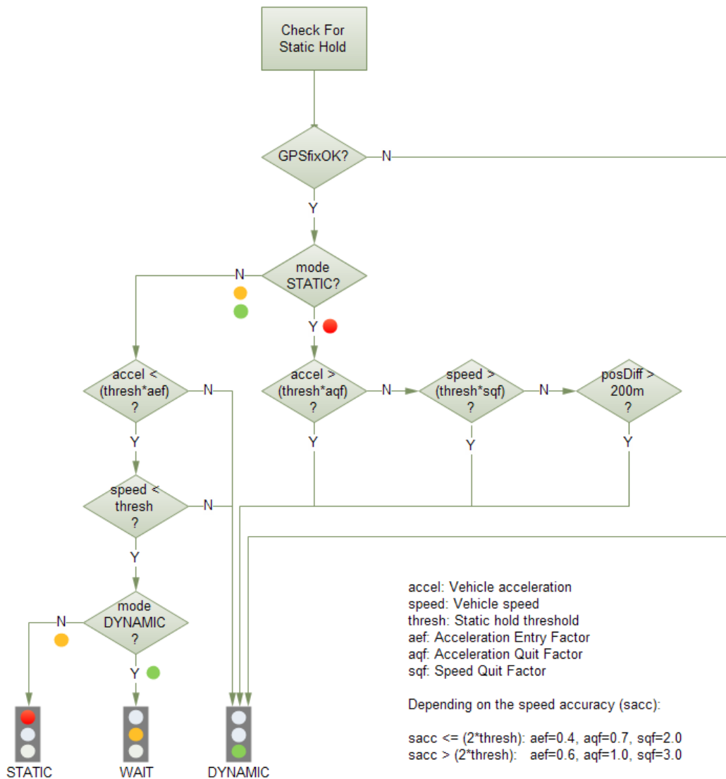
Figure 34: Flowchart of the static hold mode
