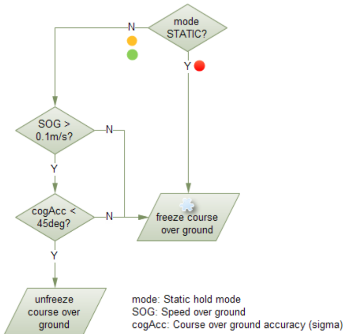
Figure 35: Flowchart of the Course Over Ground freezing
