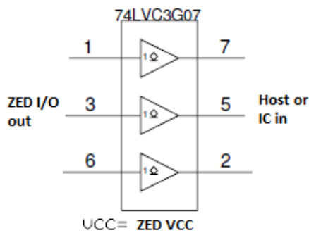
Figure 45: ZED-F9P I/O output isolation
