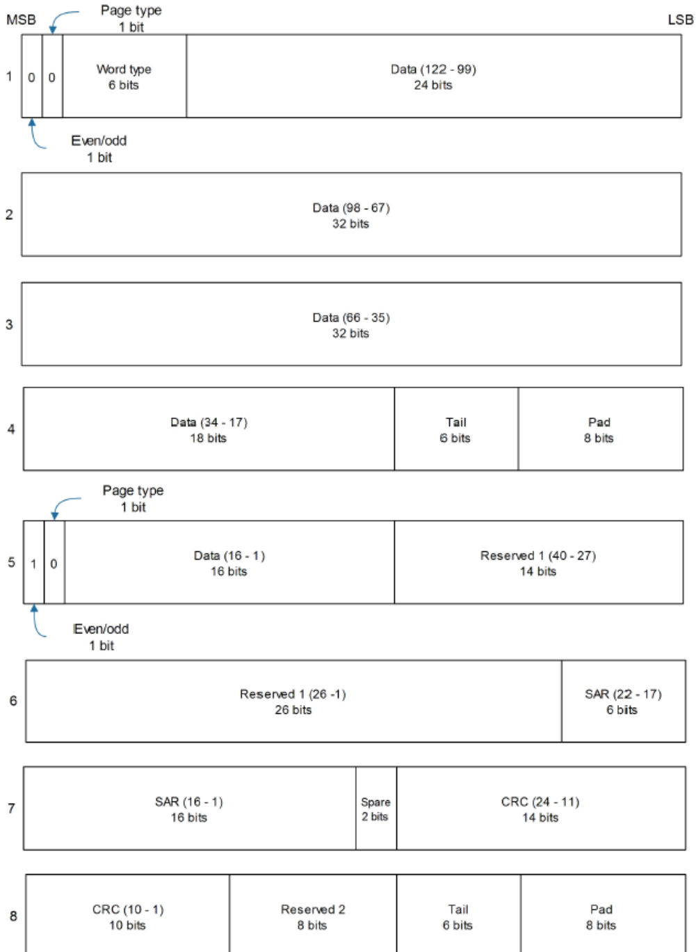
Figure 31: Galileo E1 C/B subframe words
