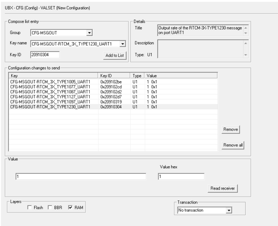
Figure 9: Base station: u-center UBX-CFG-VALSET message view for setting the CFG-MSGGOUT-* configuration group for enabling the output of the required RTCM messages
