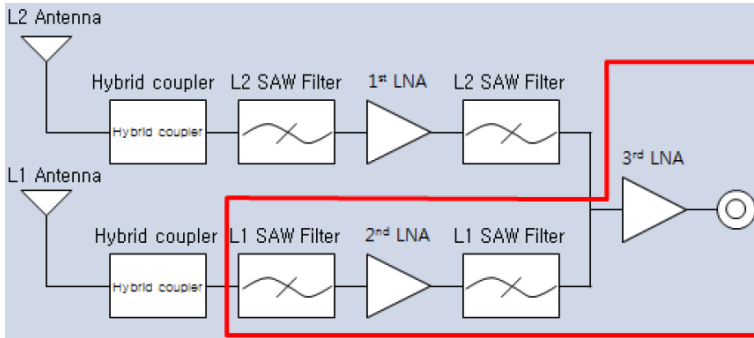
Figure 55: u-blox low cost RTK antenna internal structure
