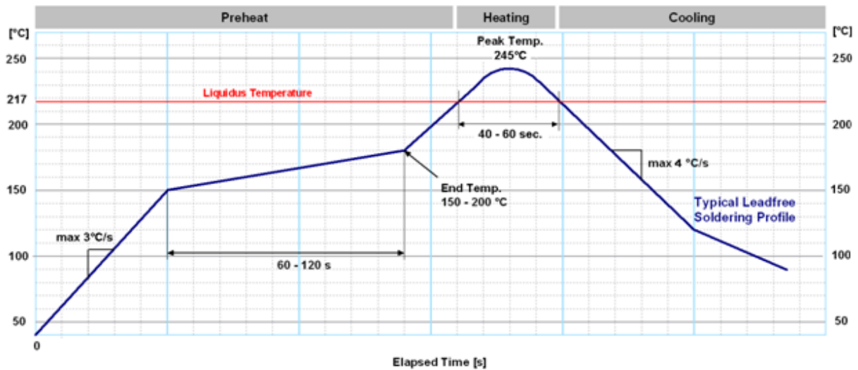
Figure 77: Soldering Profile
