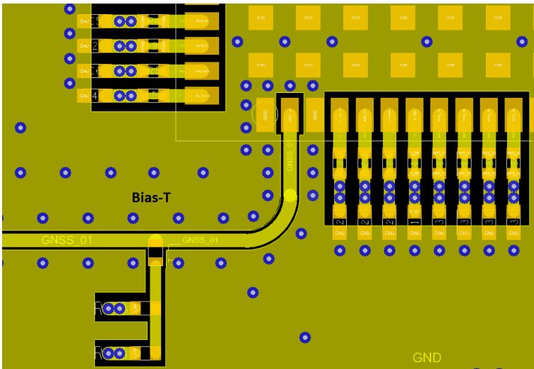
Figure 74: RF input trace
