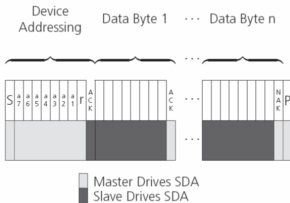
Figure 23: DDC Current Address Read Access
