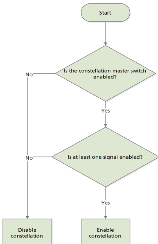
Figure 20: Flow diagram of the individual signal switches and master constellation switches
