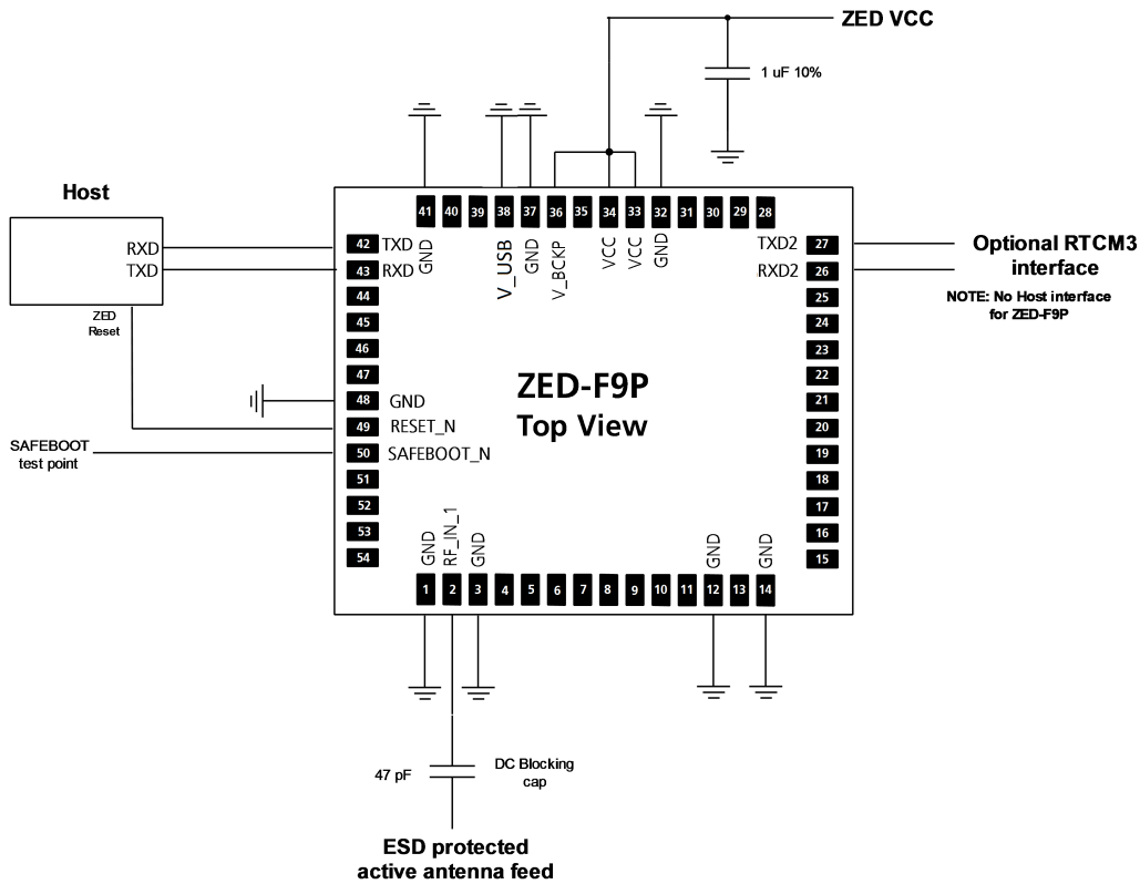
Figure 65: Minimal ZED-F9P design
