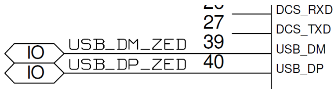
Figure 50: ZED-F9P USB_DM and USB_DP pins
