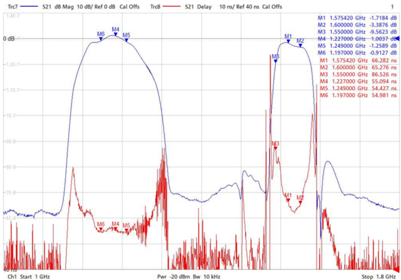
Figure 58: Low cost L1/L2 antenna Band characteristics
