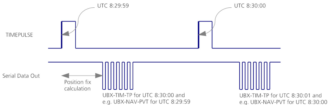
Figure 37: Timepulse and TIM-TP
