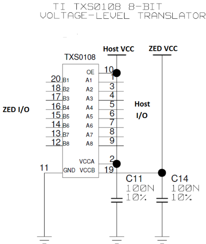
Figure 47: ZED-F9P I/O level translation
