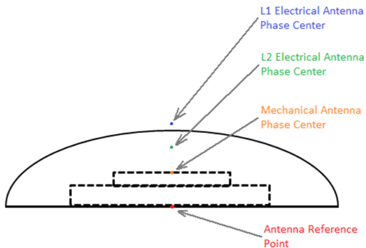
Figure 56: Stacked patch antenna
