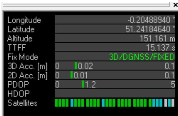
Figure 19: Rover: u-center data view with RTK Fixed
