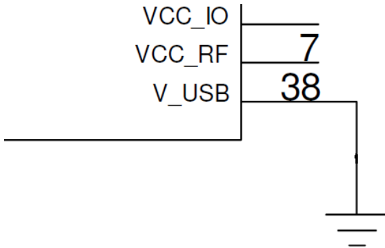
Figure 48: V_USB connected ground if not used
