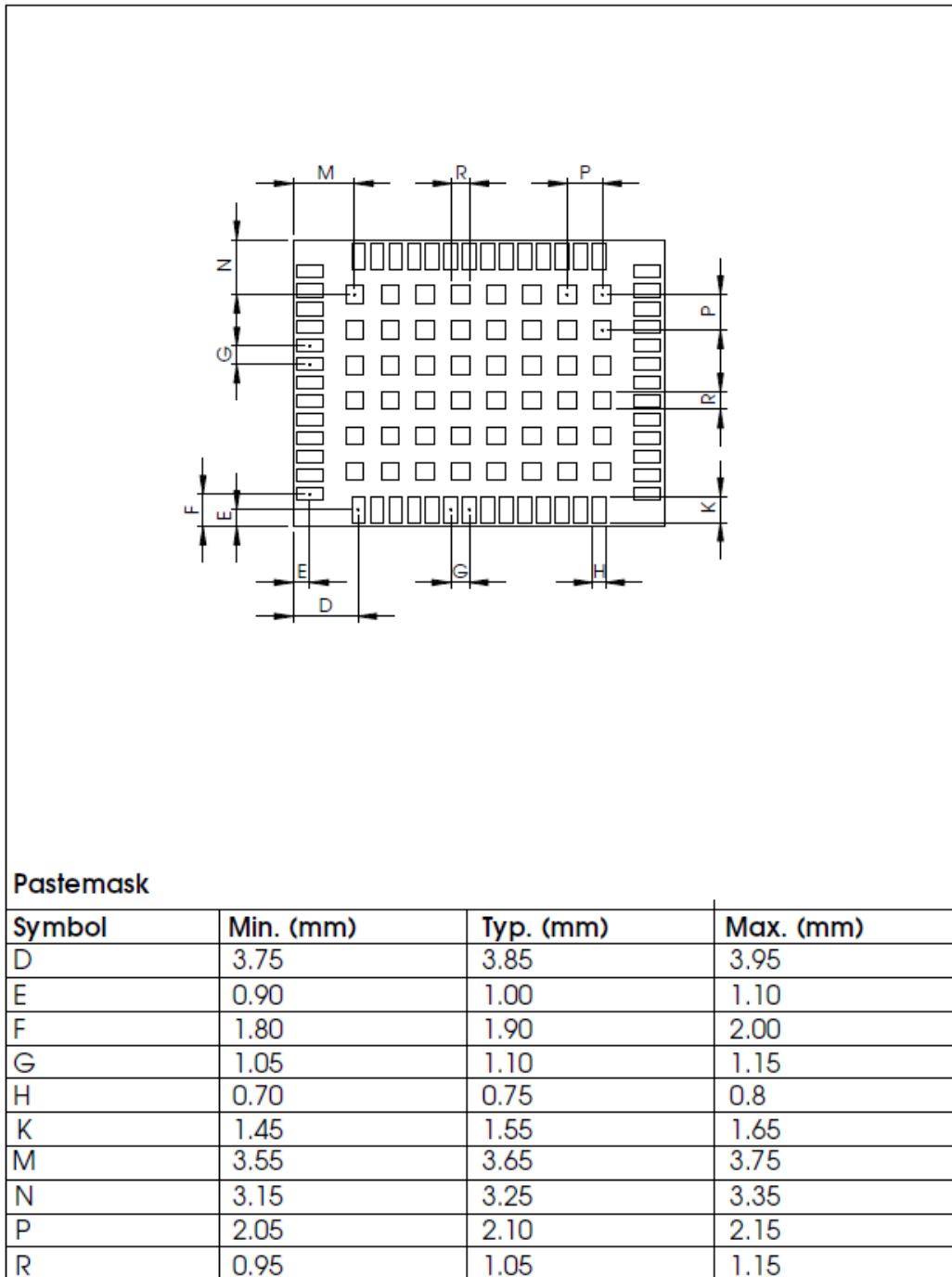
Figure 71: ZED-F9P LGA Paste mask dimensions
