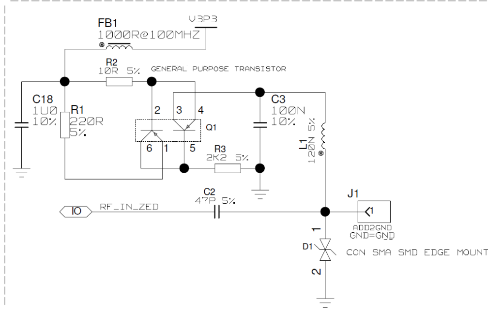
Figure 68: ZED-F9P antenna bias
