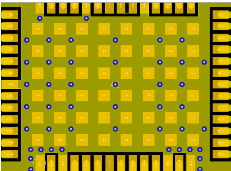
Figure 75: Top layer fill and vias
