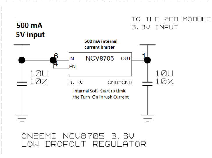
Figure 44: ZED-F9P power supply
