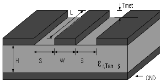
Figure 73: Grounded coplanar RF trace
