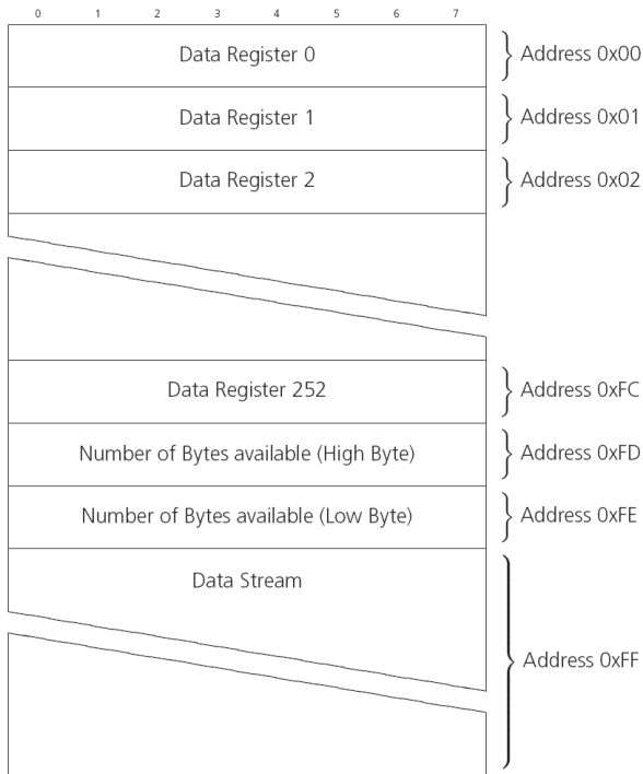
Figure 21: DDC Register Layout
