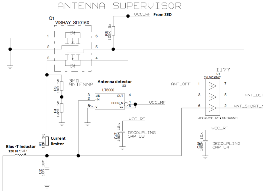
Figure 51: ZED-F9P Antenna Supervisor
