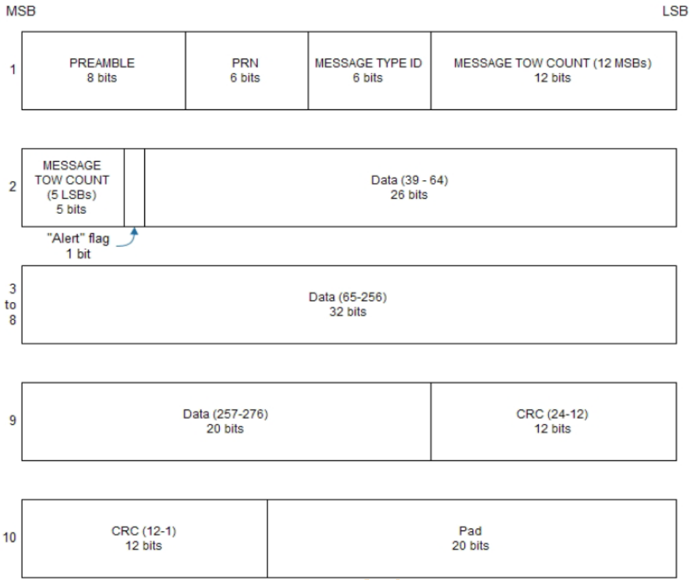
Figure 28: GPS L2C subframe words
