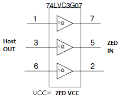
Figure 46: ZED-F9P I/O input isolation
