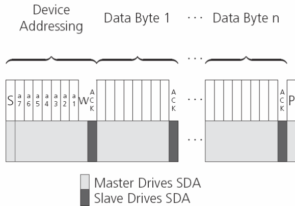
Figure 24: DDC Write Access
