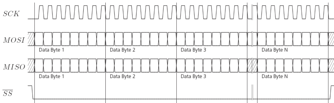
Figure 25: SPI Back-To-Back Read/Write Access
