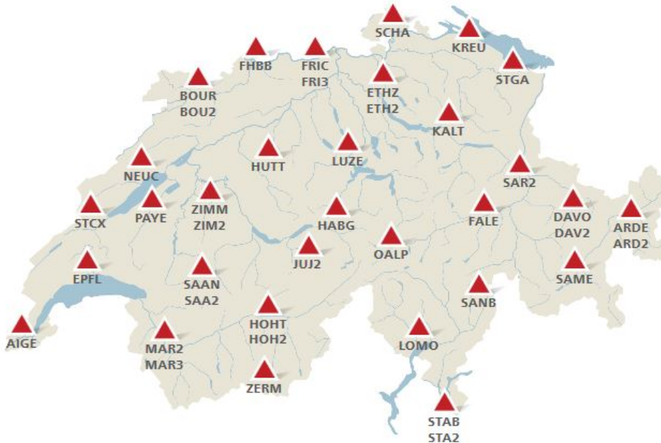
Figure 81: VRS network in Switzerland
