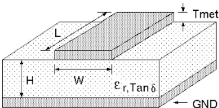
Figure 72: Microstrip trace width
