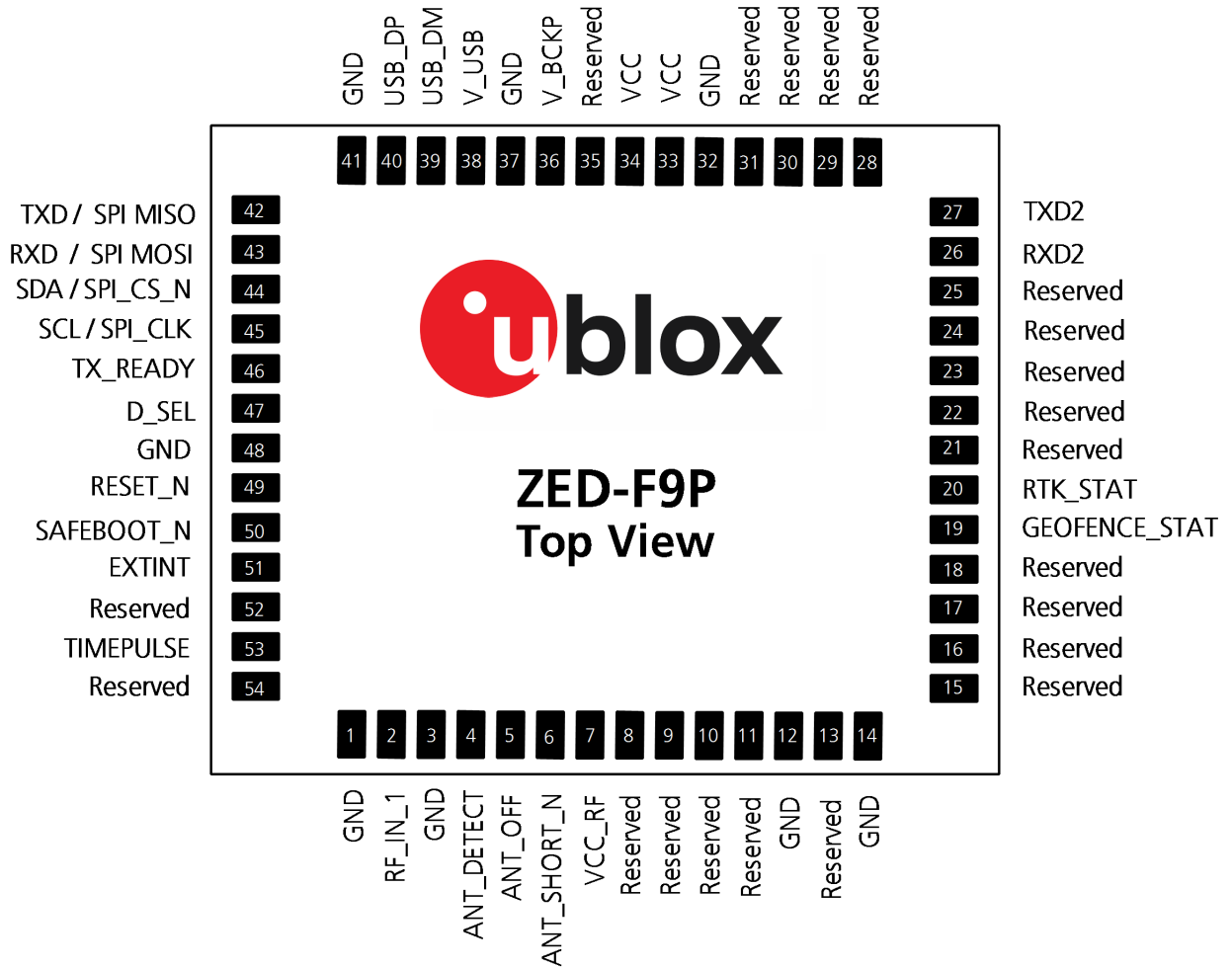
Figure 54: ZED-F9P pin assignment
