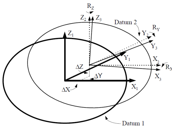
Figure 80: Transforming between two datums
