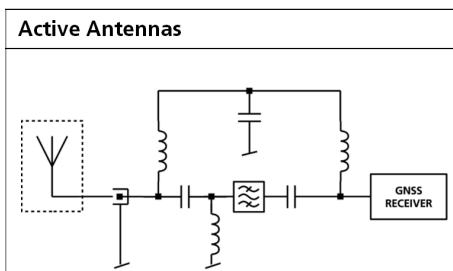
Figure 53: Active antenna EOS protection
