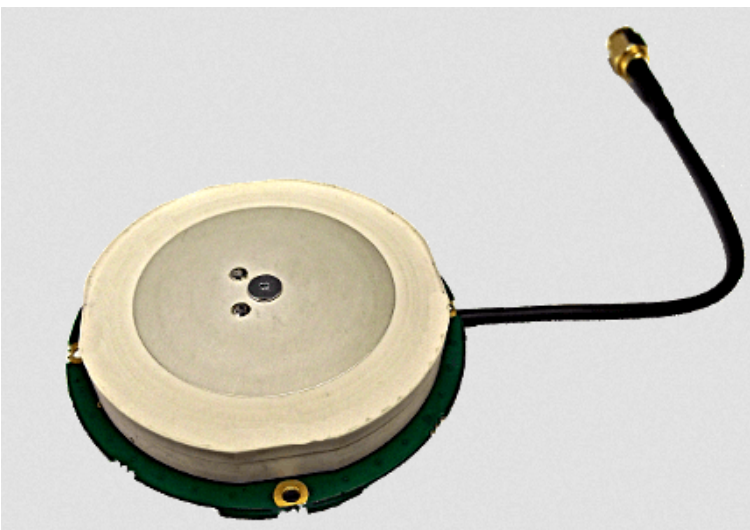
Figure 61: Tallysman active L1/L2 antenna
