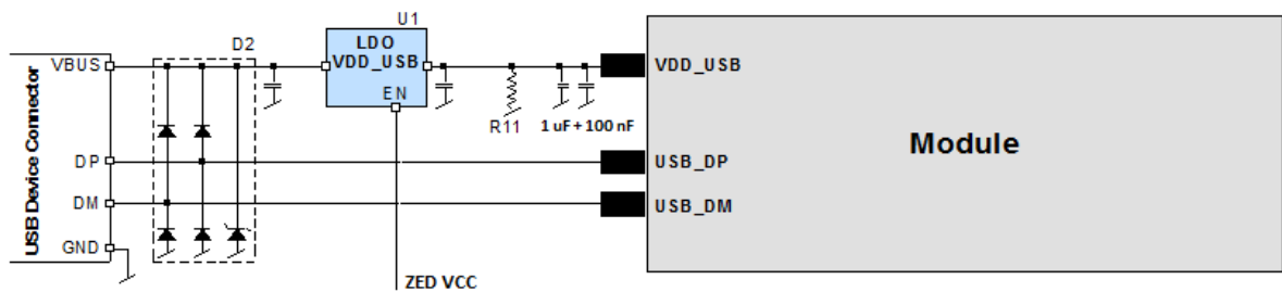
Figure 49: ZED-F9P V_USB supply
