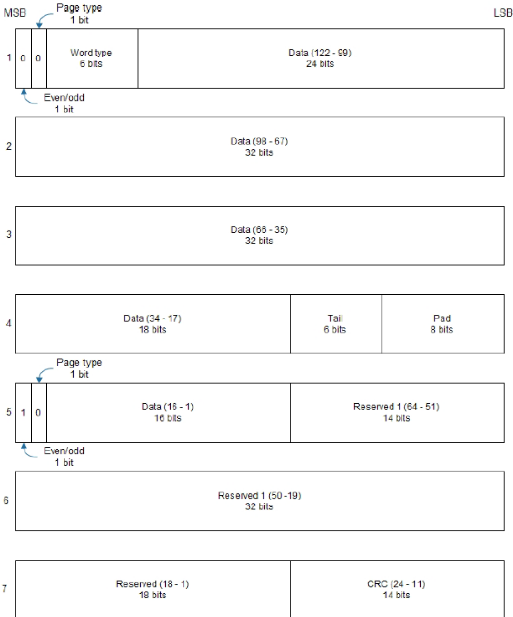
Figure 32: Galileo E5 b1/bQ subframe words
