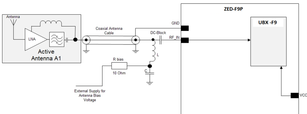
Figure 67: ZED-F9P external voltage antenna bias
