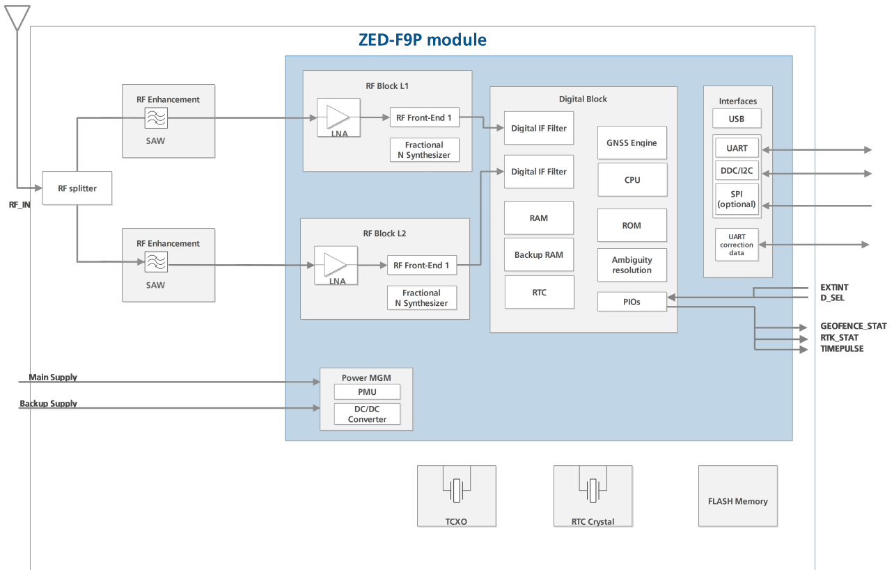
Figure 43: ZED-F9P block diagram
