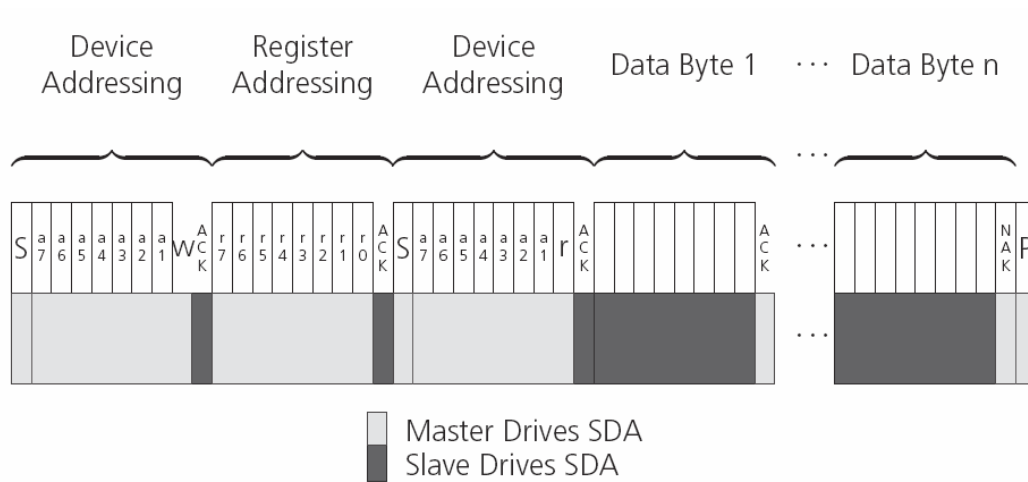
Figure 22: DDC Random Read Access
