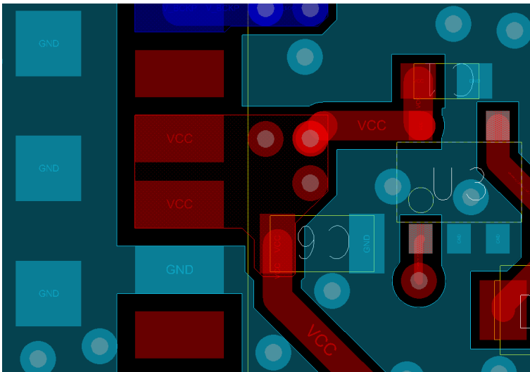
Figure 76: VCC pads
