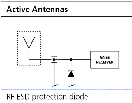
Figure 52: RF ESD precautions
