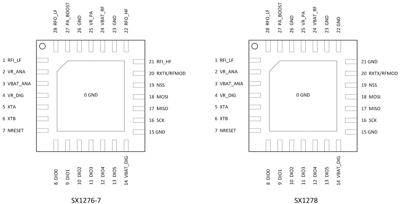
Figure 2. Pin Diagrams
