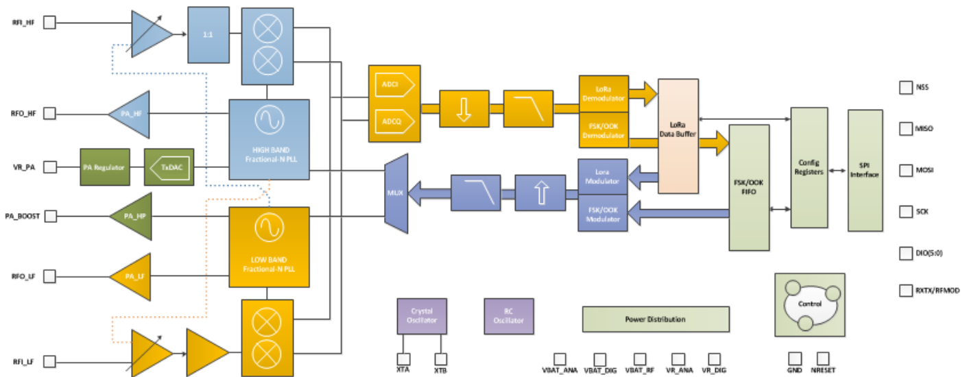
Figure 3. SX1276/77/78 Block Schematic Diagram
