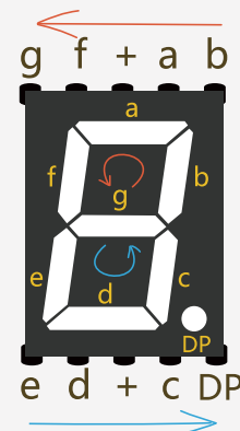
Fig. 15-2 Pin-out Instructions
