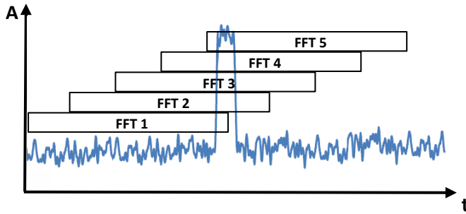
Figure 7: Overlapping process in real-time spectrum analyzer
