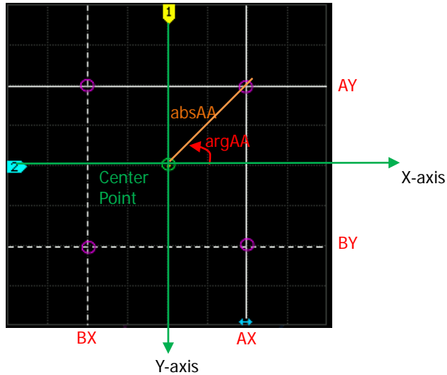
Figure 6-8 XY Cursor Measurement Definition
