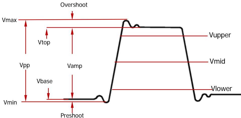
Figure 6-5 Voltage Parameters
