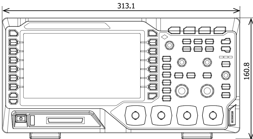
Figure 1-1 Front View
